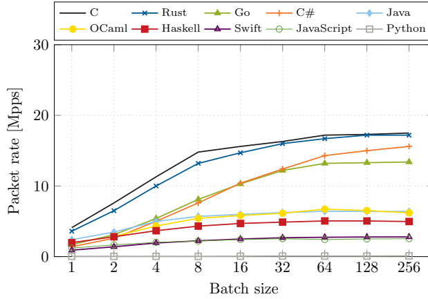
(a) Forwarding rate on 1.6 GHz CPU
